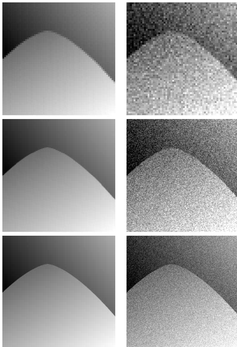
Figure 2. (Left) \delta^n f , for n = 64, 128, 256 , respectively, where f is a horizon function, according to Definition 2. Here, the horizon boundary is in \mathcal{C}^\alpha((0, 1)) and \alpha = 1.5 ; (Right) Respective noisy images \delta^n f + \xi^n .
