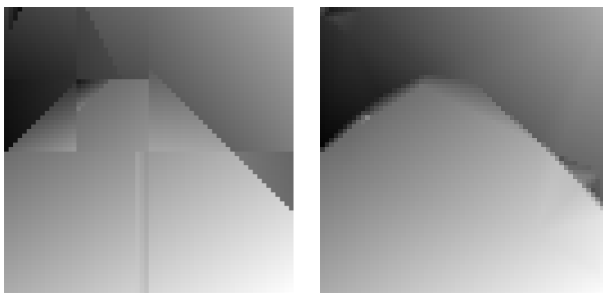
Figure 3. Estimators of the noisy images of Figure 2. (Left) piecewise linear wedgelet estimator; (Right) piecewise linear and continuous Delaunay estimators.
